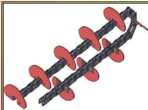
REDLER- TRANSGRAN (CHAIN CONVEYORS/CON- VOYEURS A CHAIN)
